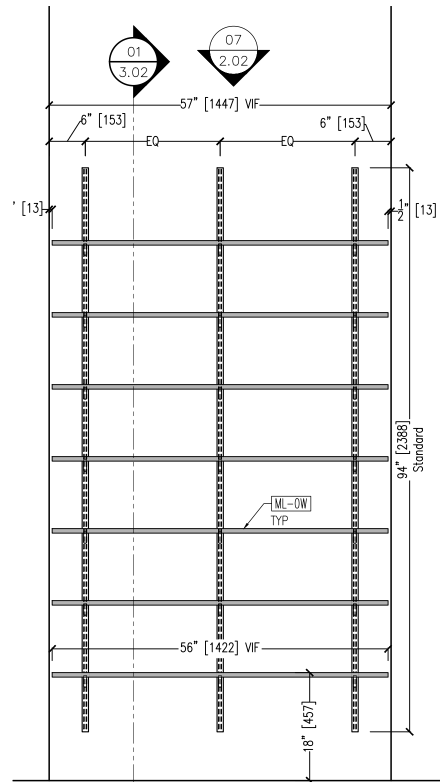
06 ELEVATION B @ STORAGE MW05A 2.02 SCALE: 3/4" = 12" ARCH. REF.:10/8.02
