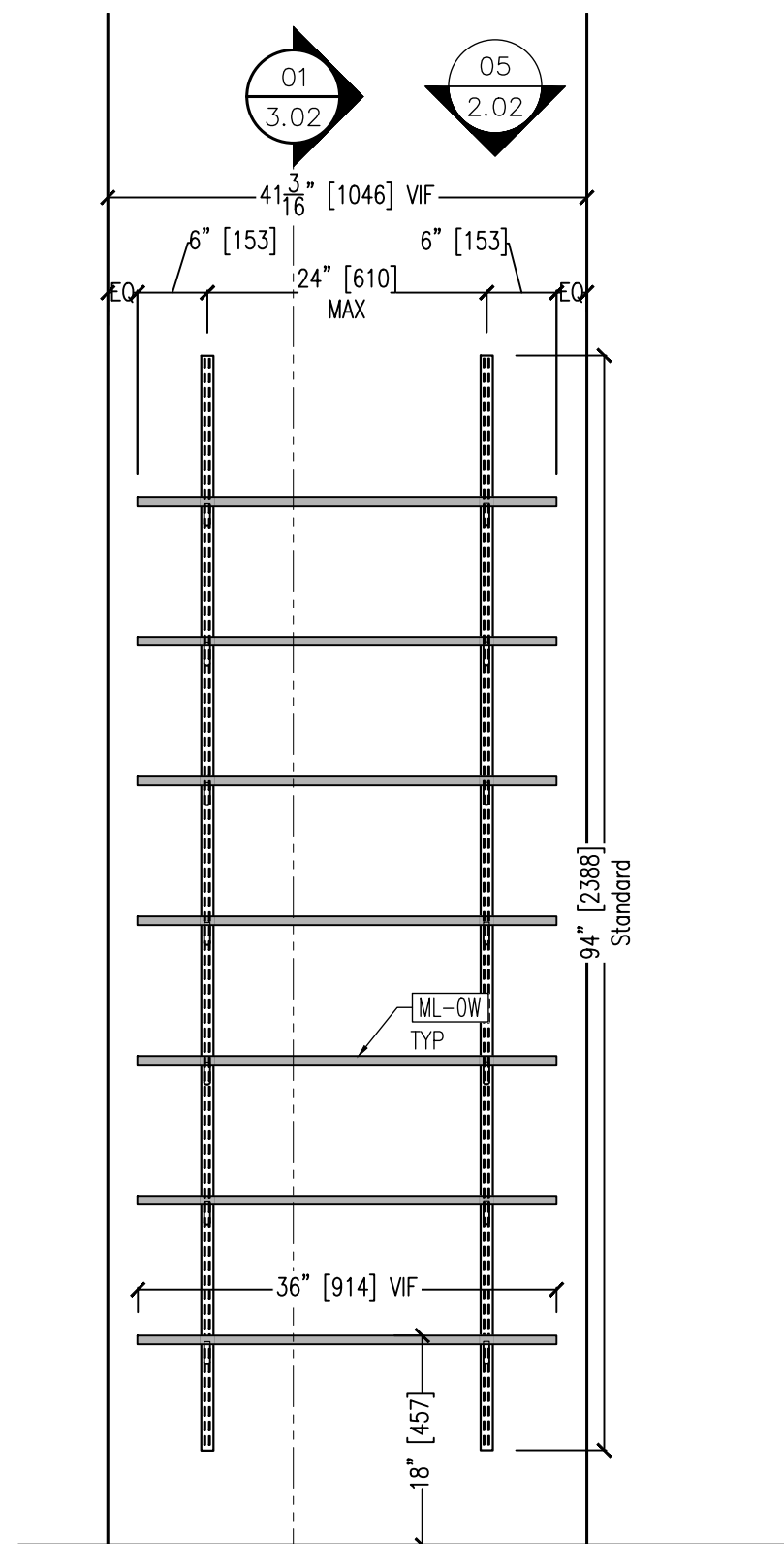
04 ELEVATION A @ STORAGE MW05B 2.02 SCALE: 3/4" = 12" ARCH. REF.:9/8.02
