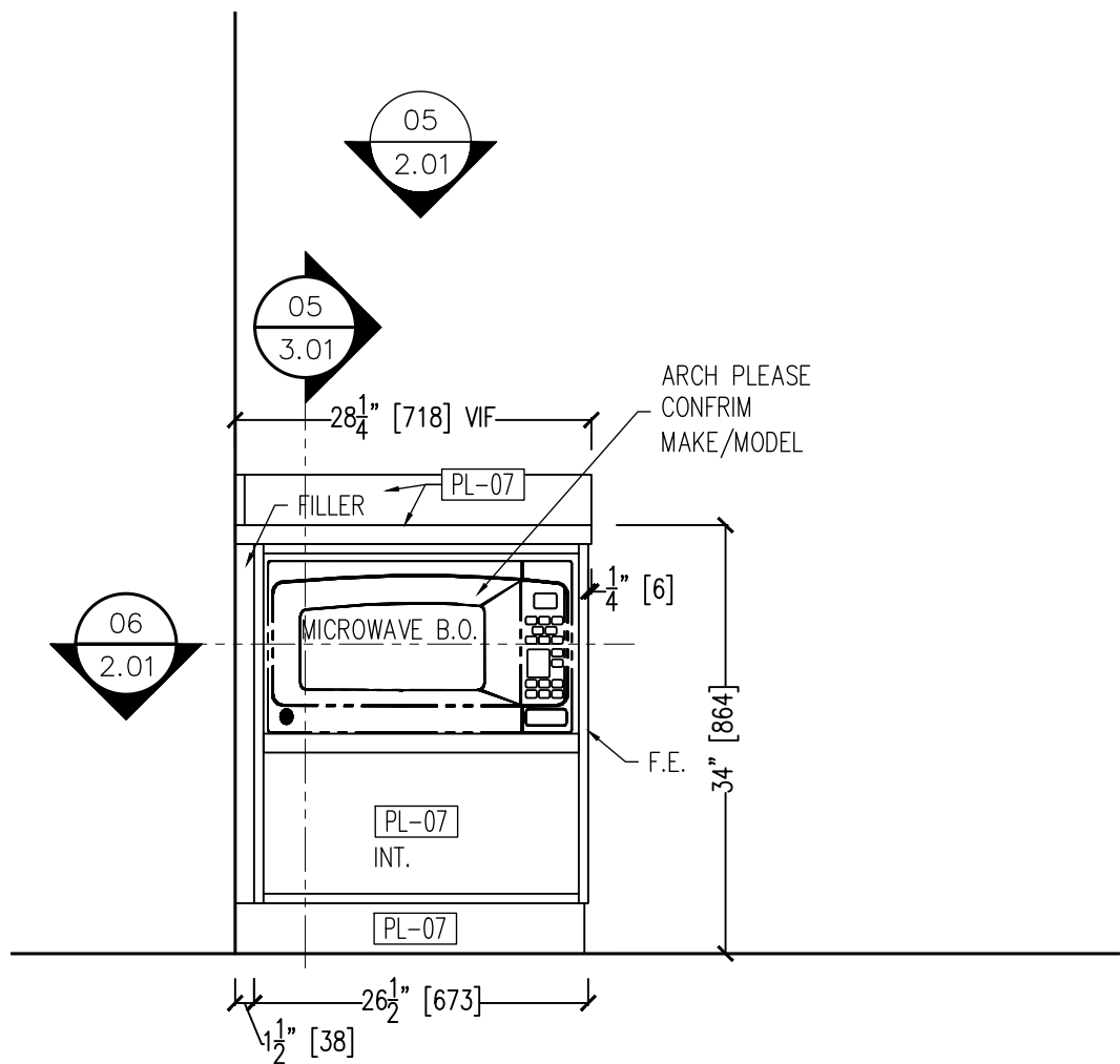
04 ELEVATION @ BREAK/Wellness 2.01 SCALE: 3/4" = 12" ARCH. REF.:14/8.02
