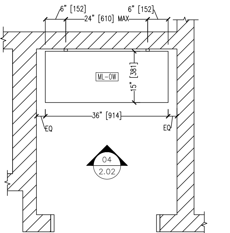
05 PLAN @ STORAGE MW05B 2.02 SCALE: 3/4" = 12" ARCH. REF.:0/0.00
