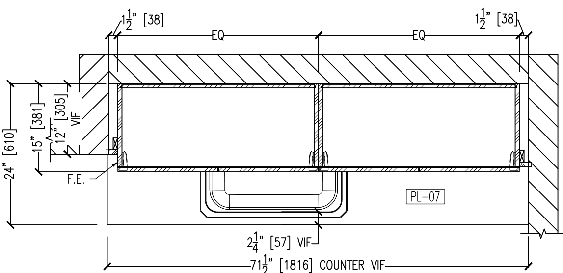
02 UPPER PLAN @ BREAK/Wellness 2.01 SCALE: 3/4" = 12" ARCH. REF.:0/0.00
