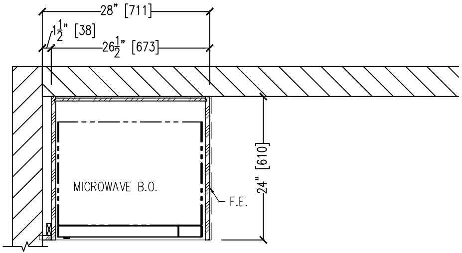
06 LOWER PLAN @ BREAK/Wellness 2.01 SCALE: 3/4" = 12" ARCH. REF.:0/0.00
