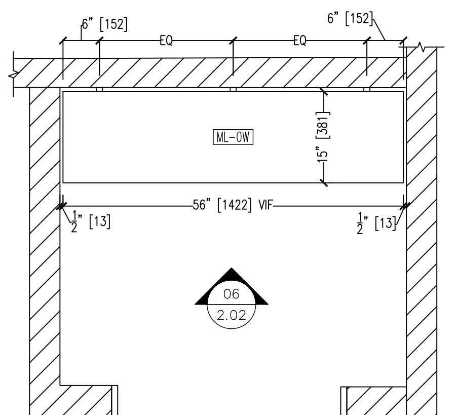
07 PLAN @ STORAGE MW05A 2.02 SCALE: 3/4" = 12" ARCH. REF.:0/0.00
