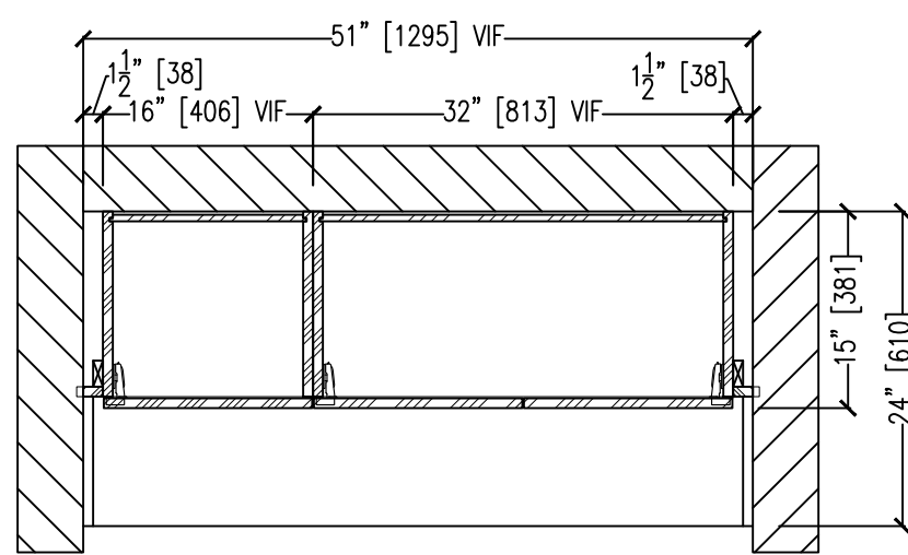
08 UPPER PLAN BEHIND CSR 2.01 SCALE: 3/4" = 12" ARCH. REF.:0/0.00
