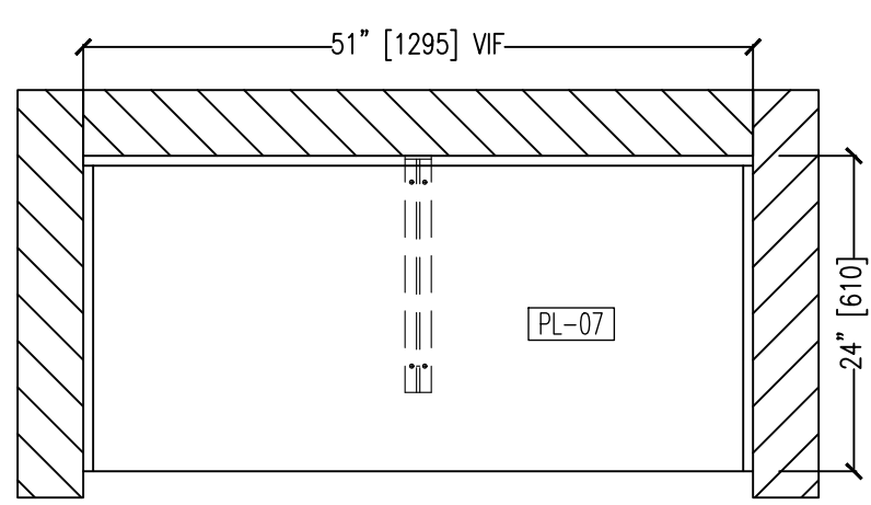
09 COUNTER PLAN BEHIND CSR 2.01 SCALE: 3/4" = 12" ARCH. REF.:0/0.00
