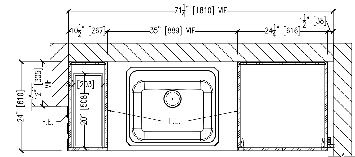
03 LOWER PLAN @ BREAK/Wellness 2.01 SCALE: 3/4" = 12" ARCH. REF.:0/0.00
