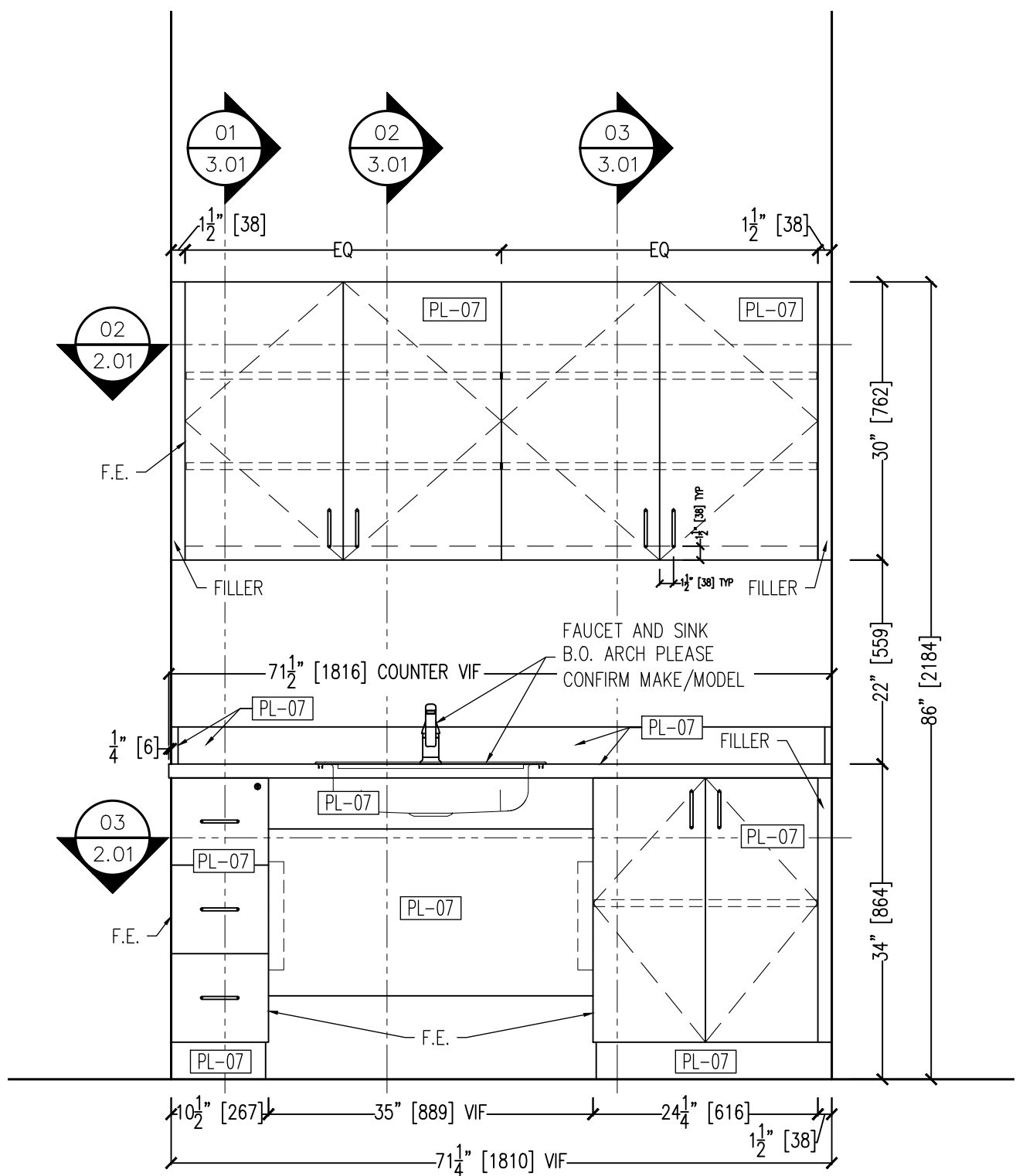
01 ELEVATION @ BREAK/Wellness 2.01 SCALE: 3/4" = 12" ARCH. REF.:13/8.02
