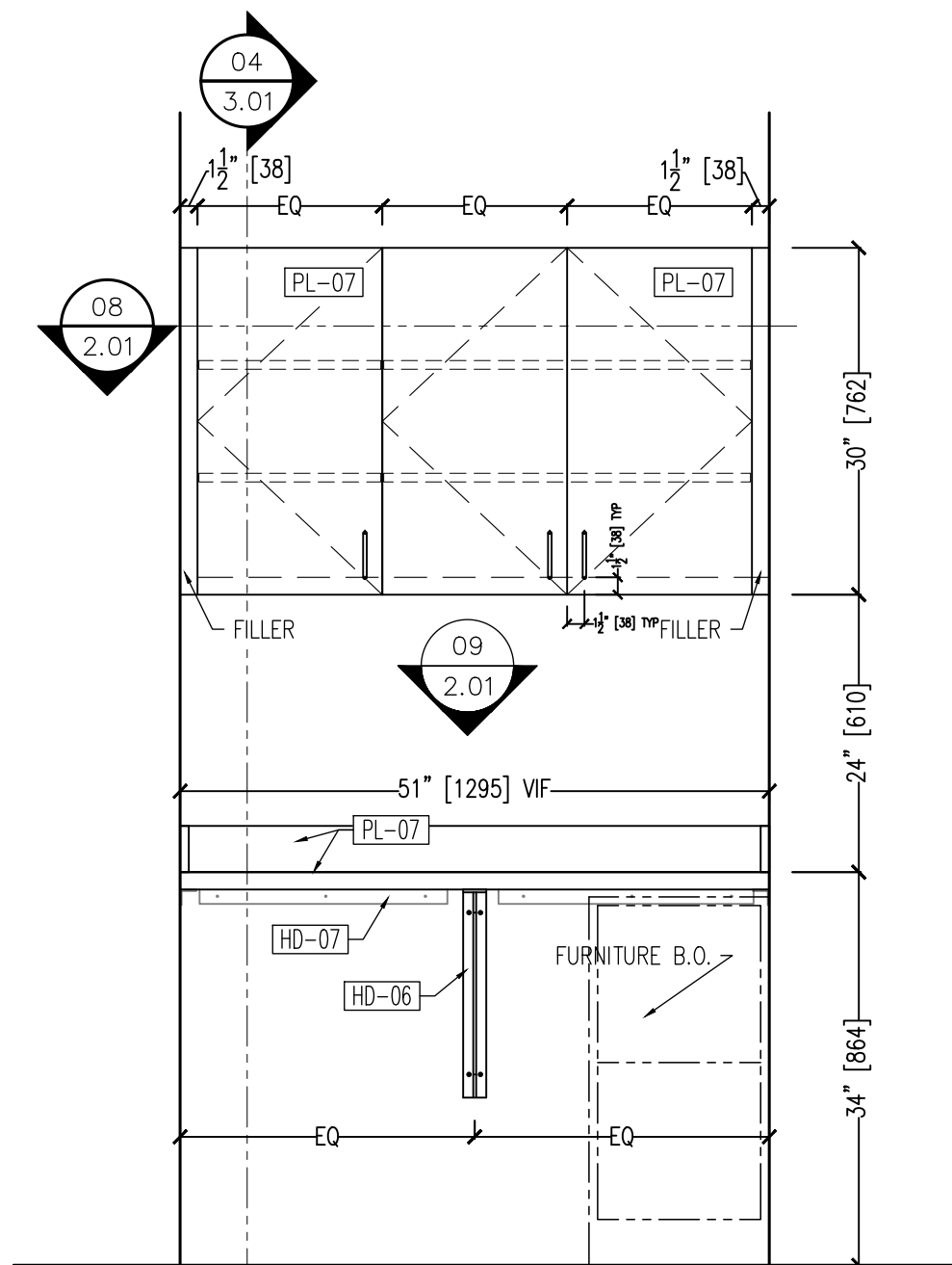
07 ELEVATION A BEHIND CSR 2.01 SCALE: 3/4" = 12" ARCH. REF.:0/0.00
