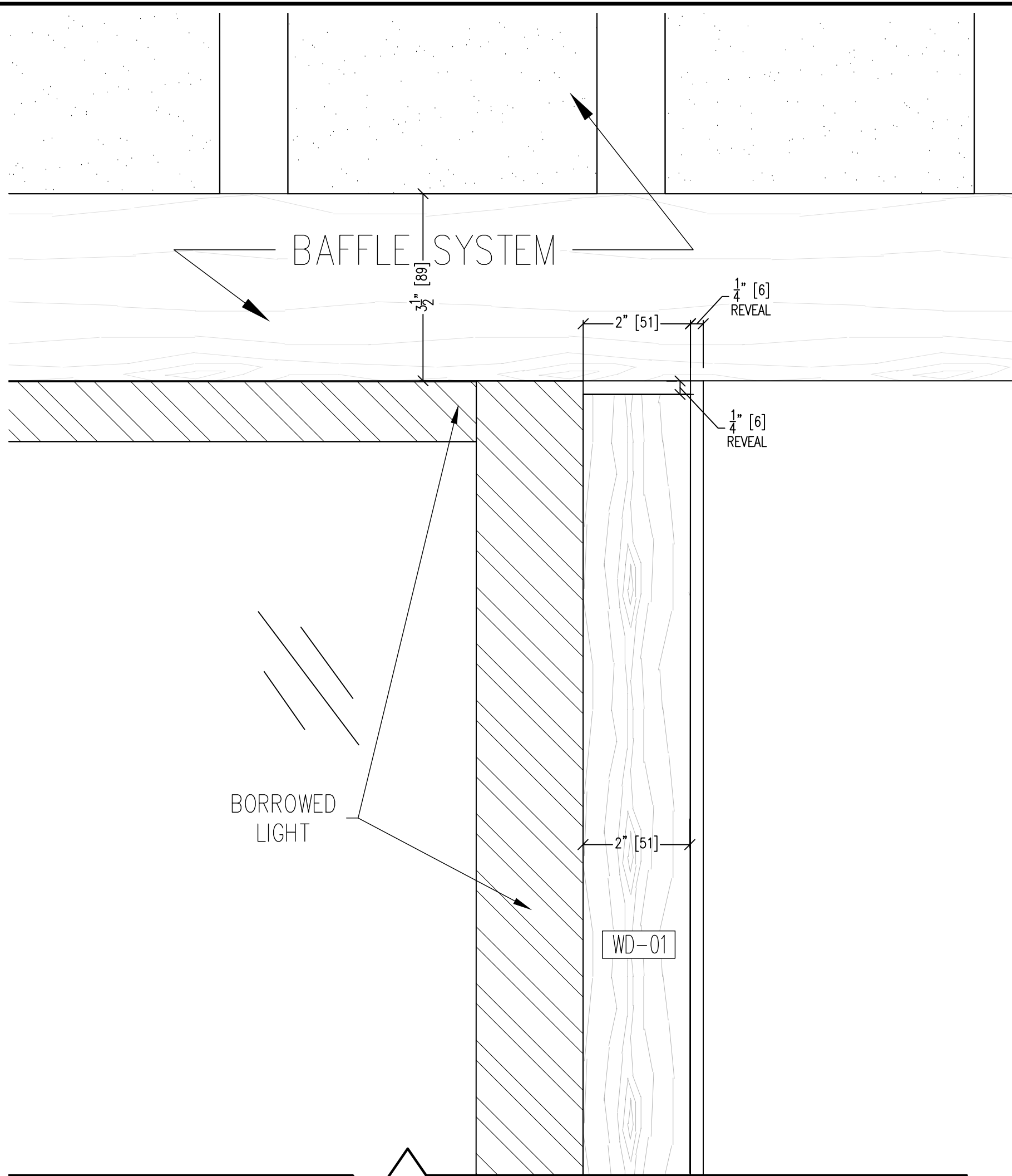
08 BLOW-UP SECTION @ BORROWED LIGHT - GRAB & GO SIDE - RIGHT END 2.12 SCALE: 6" = 12" ARCH. REF.:
