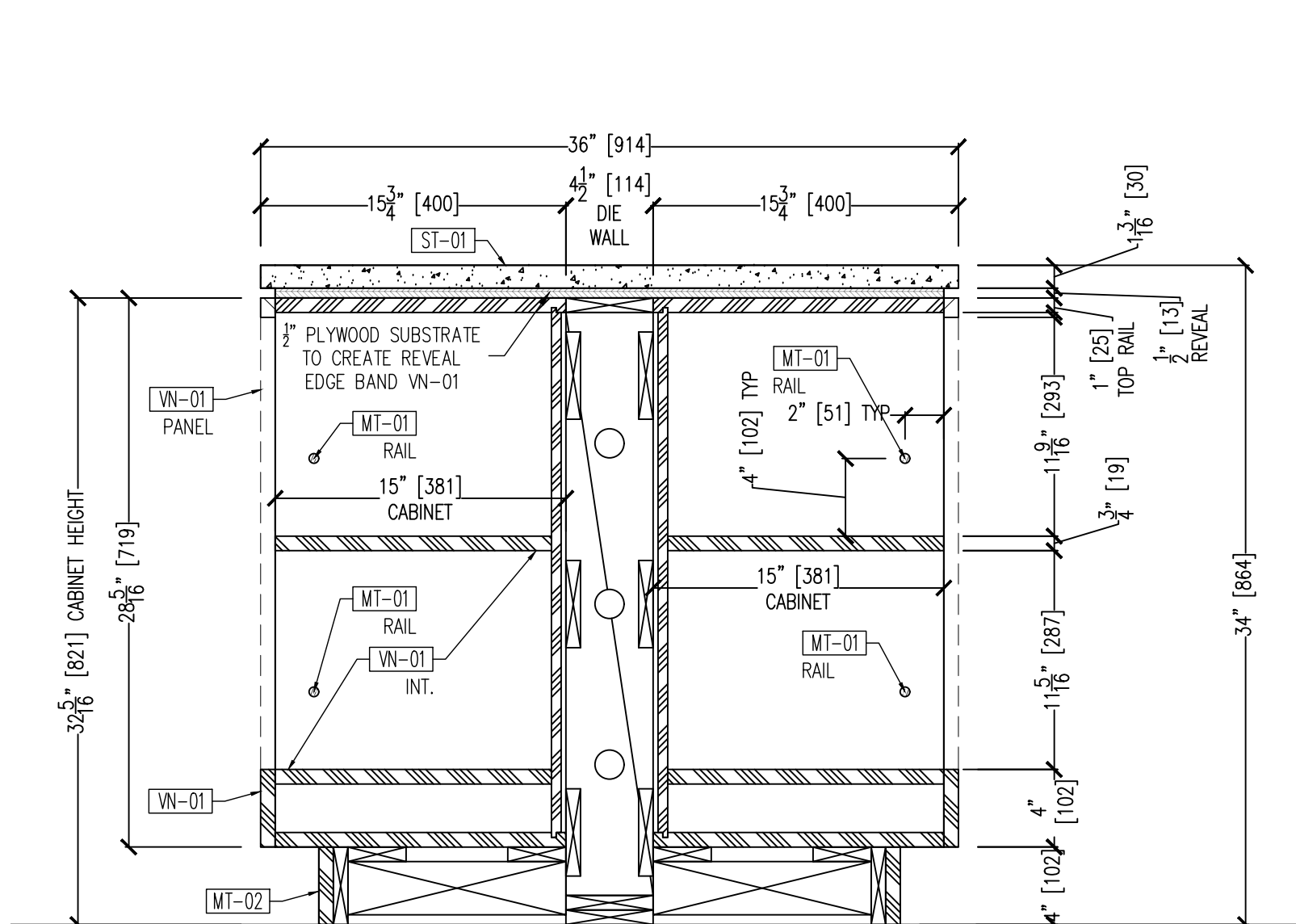
03 SECTION @ SNACK BAR ISLAND - (2 REQUIRED) 3.03 SCALE: 1 1/2" = 12" ARCH. REF.:12/552
