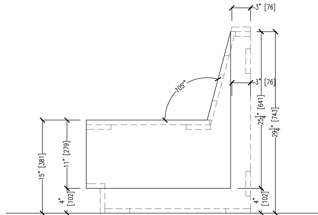
08 SECTION @ APPLIED ENDS @ ENS OF BENCHES 3.06 SCALE: 1 1/2" = 12" ARCH. REF.:32/541
