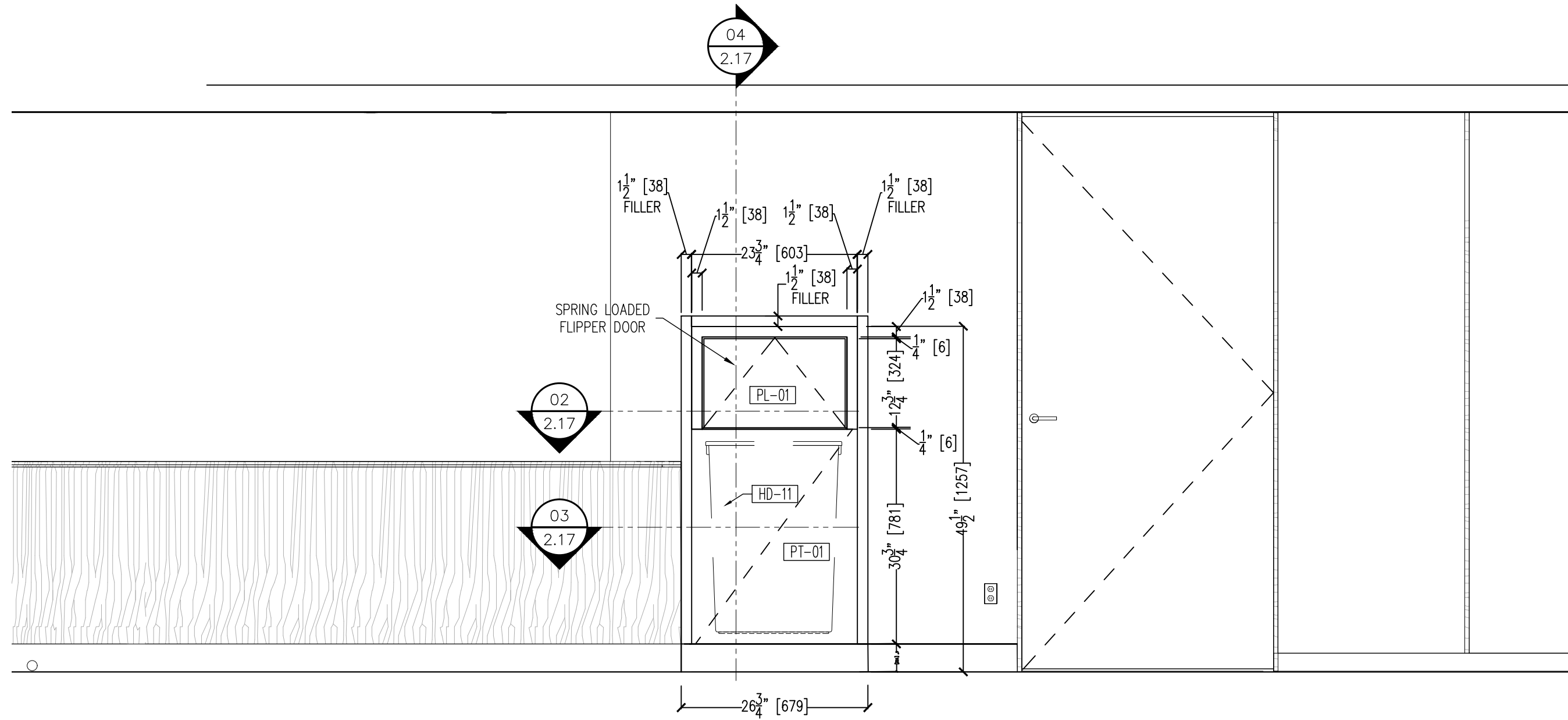
01 ELEVATION @ SECOND MARKET ENTRY - SOUTHEAST 2.17 SCALE: 3/4" = 12" ARCH. REF.:200B.00/42
