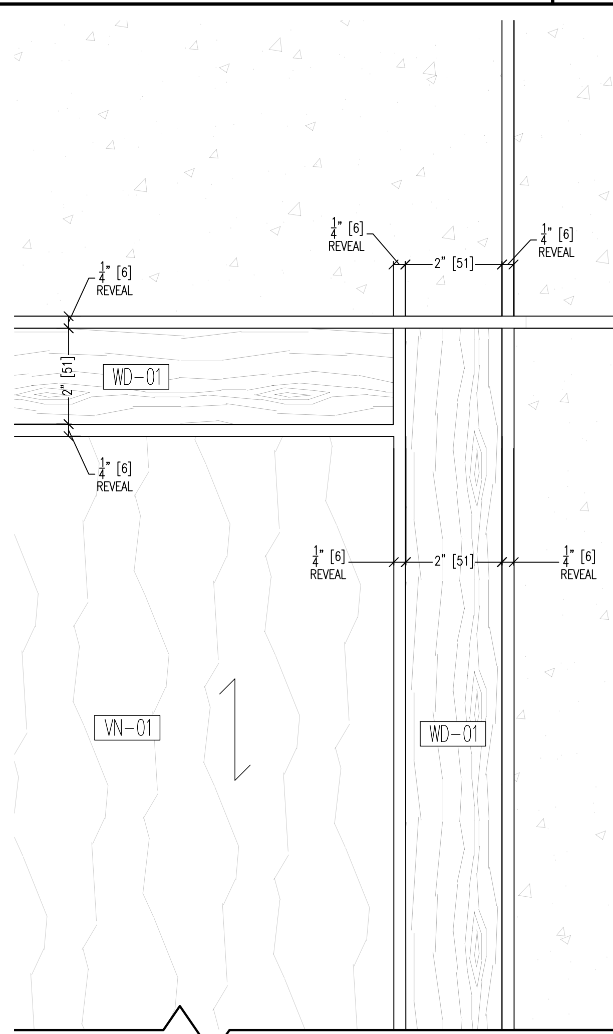
08 BLOW-UP SECTION @ BORROWED LIGHT - GRAB & GO SIDE - RIGHT END 2.12 SCALE: 6" = 12" ARCH. REF.:
