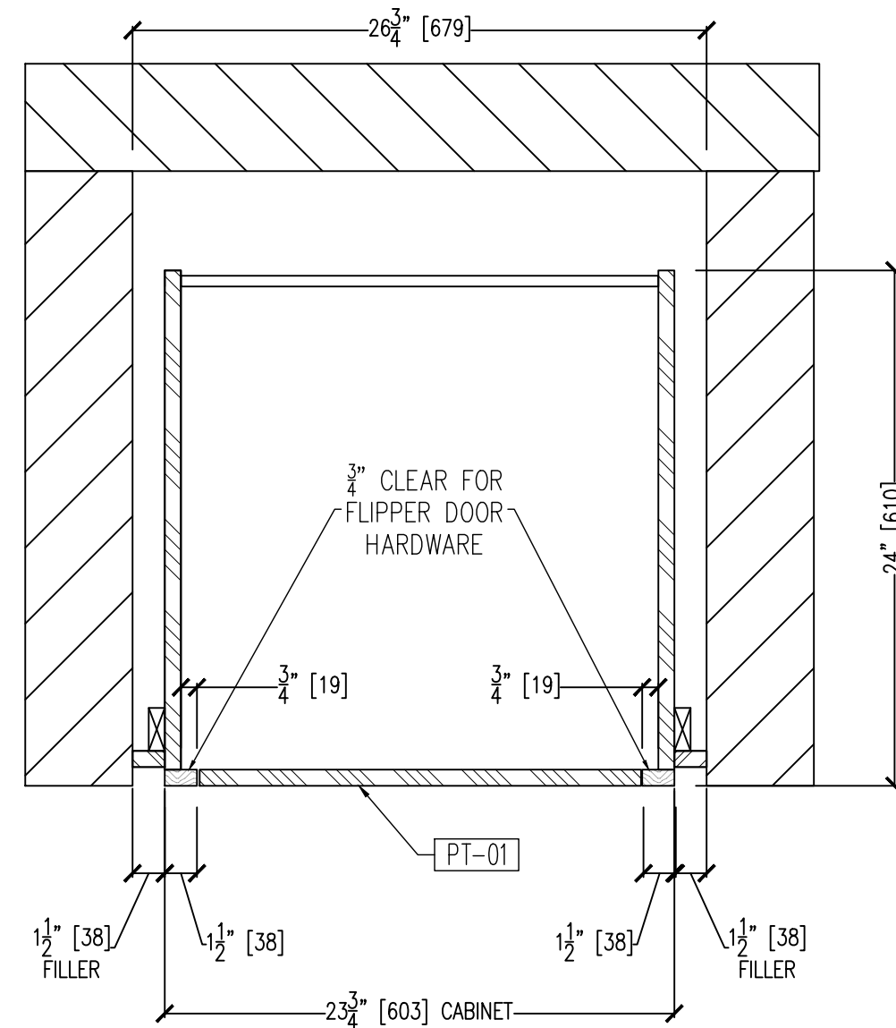
01 UPPER PLAN @ MARKET SECONDARY ENTRY 2.17 SCALE: 1-1/2" = 12" ARCH. REF.:A-200B.00 / 41
