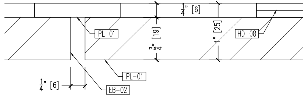
07 DETAIL @ REVEAL 3.02 SCALE: 12" = 12" ARCH. REF.00/0.00
