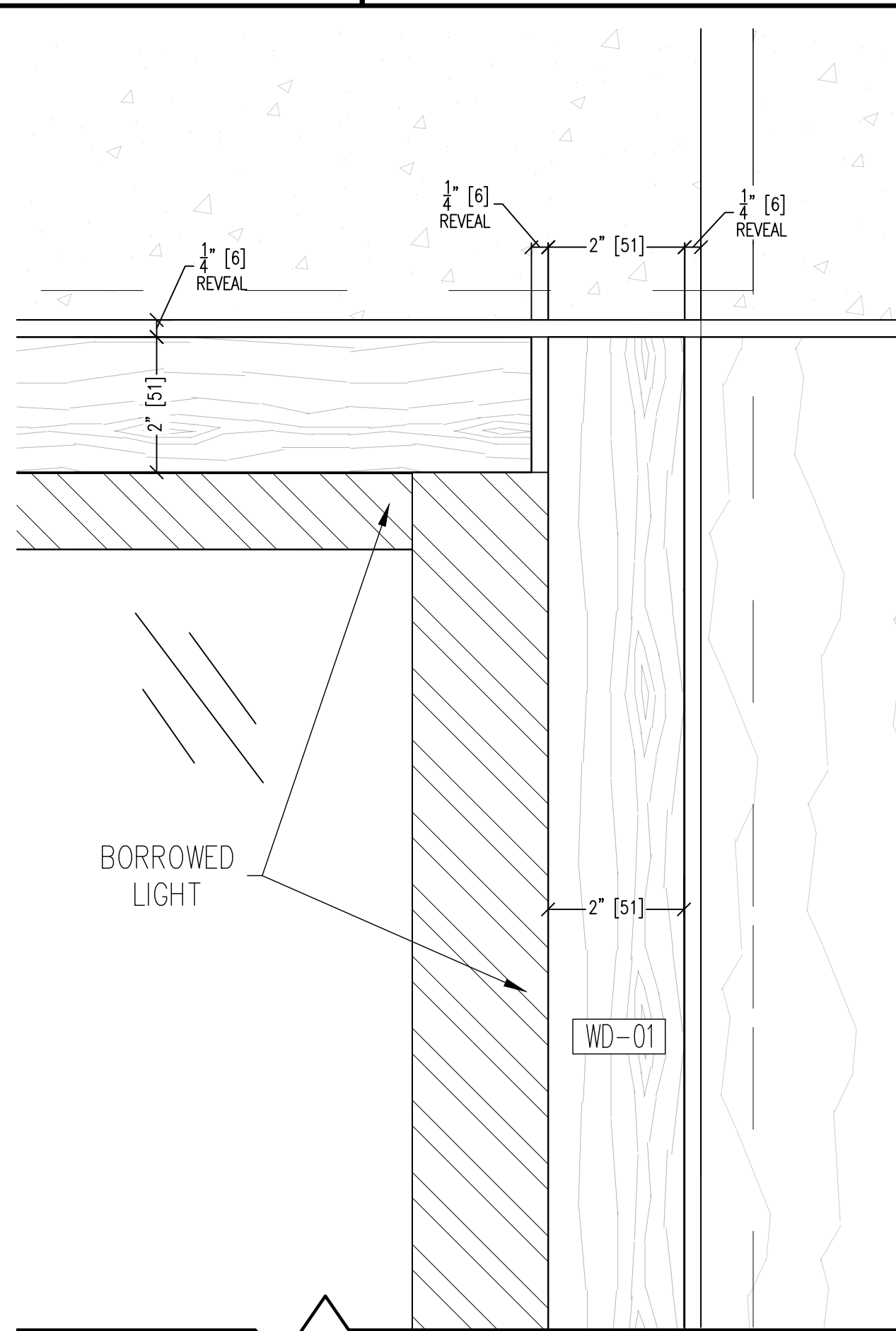
03 BLOW-UP SECTION @ MIDDLE END PANEL 2.12 SCALE: 6" = 12" ARCH. REF.:
