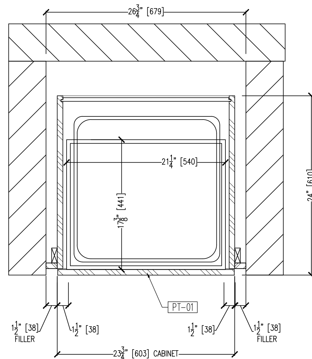
02 LOWER PLAN @ MARKET SECONDARY ENTRY 2.17 SCALE: 1-1/2" = 12" ARCH. REF.:A-200B.00 / 41
