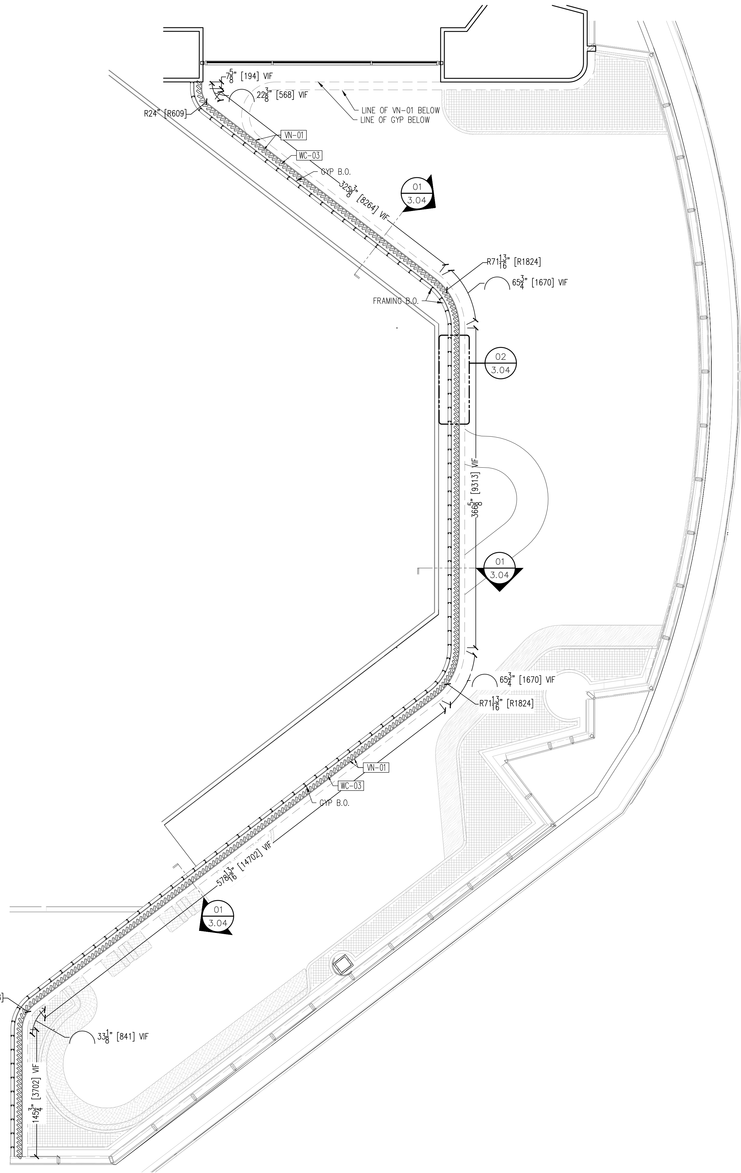
02 PLAN @ LOWER BAFFLE SYSTEM 2.15 SCALE: 3/16" = 12" ARCH. REF.:11/405
