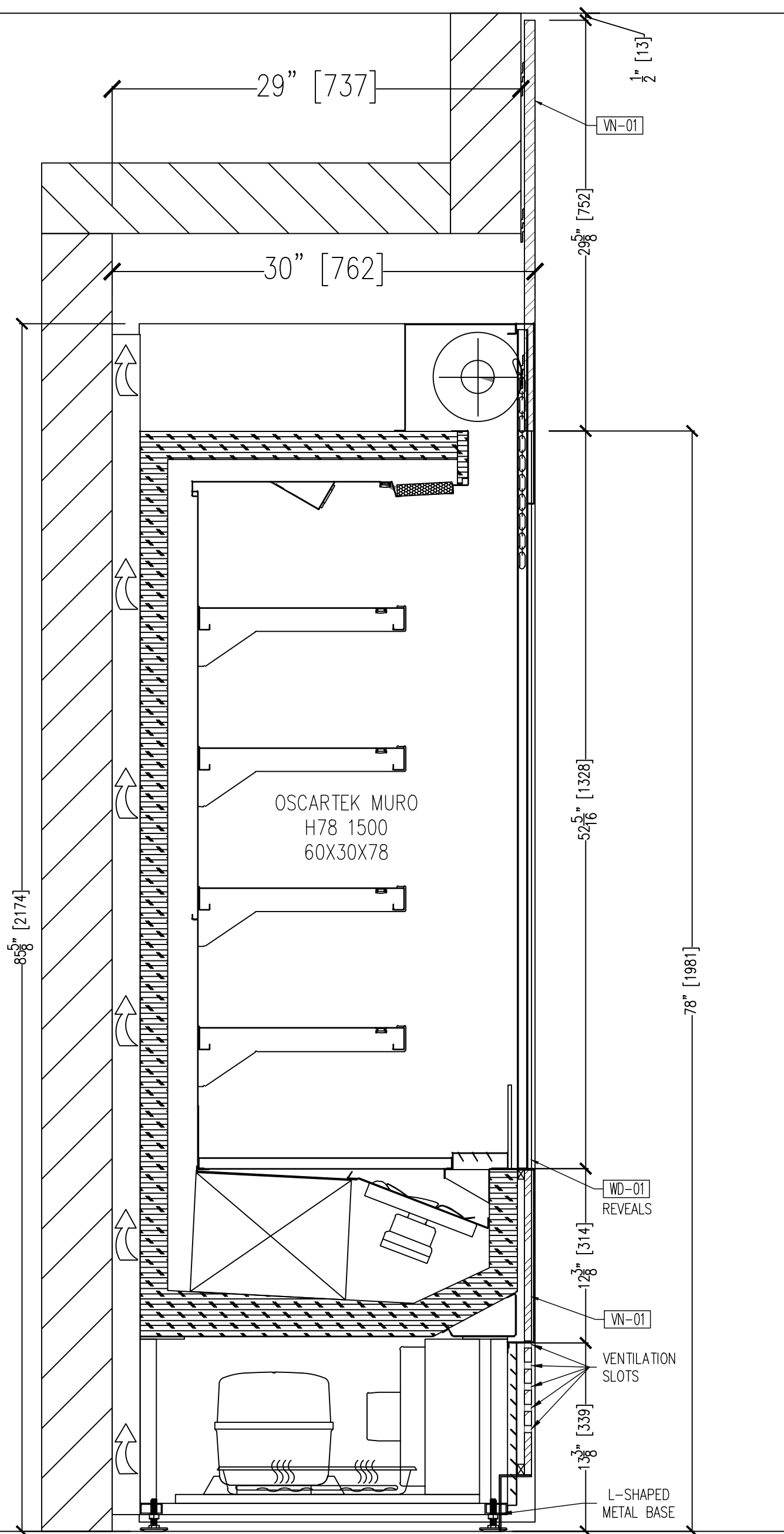
01 SECTION @ FRIDGE SHOWCASE 3.03 SCALE: 1 1/2" = 12" ARCH. REF.:11/552
