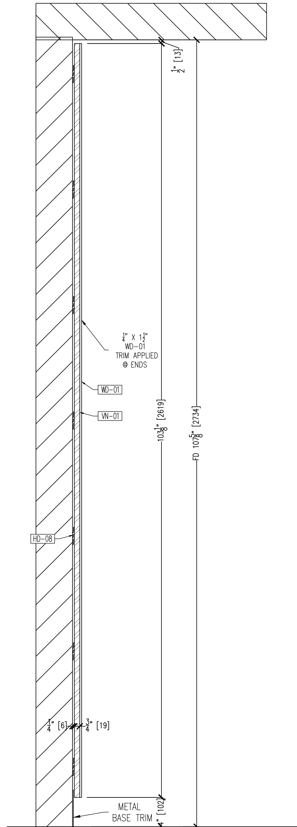
04 SECTION @ TYPICAL WALL PANEL 3.02 SCALE: 1 1/2" = 12" ARCH. REF.0/0.00
