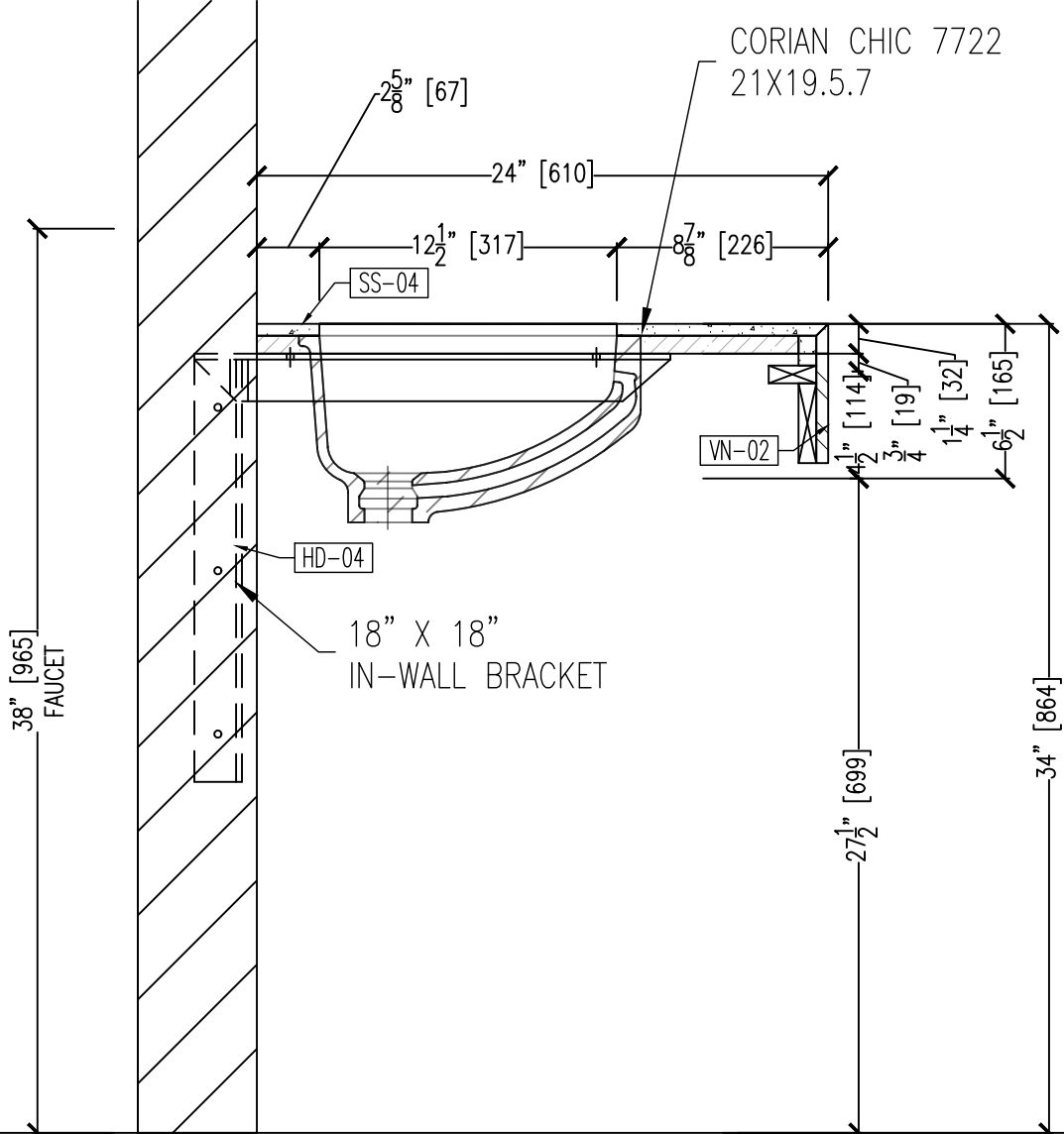
06 SECTION @ ADA BATHROOM 3.03 SCALE: 1 1/2" = 12" ARCH. REF.:31/552
