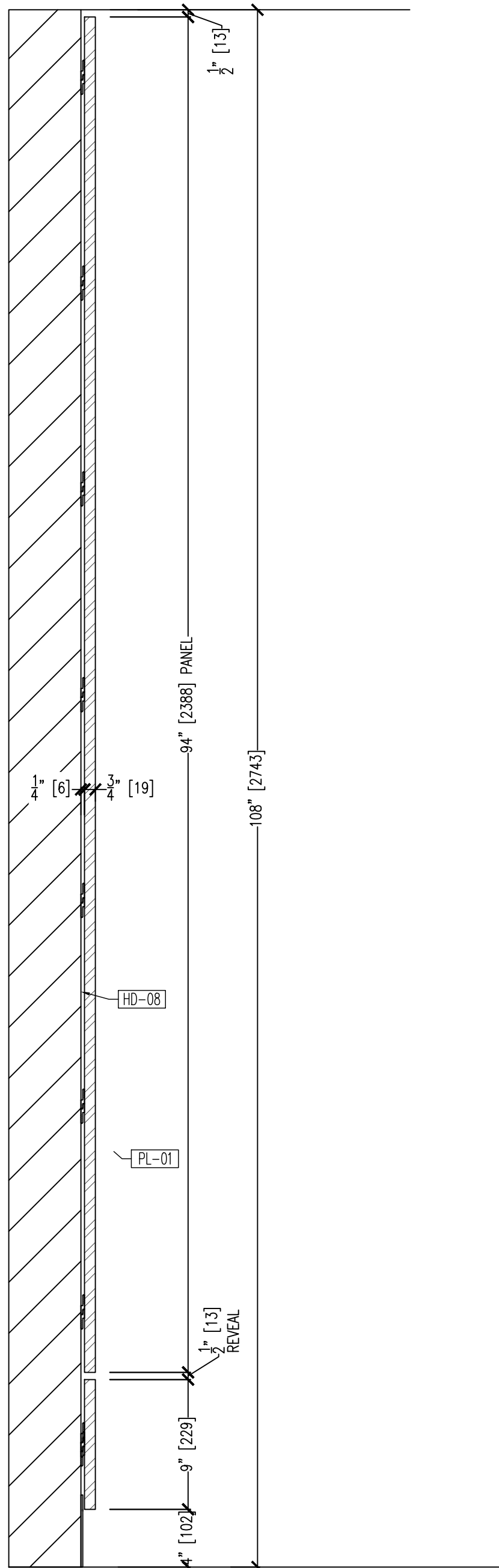
01 SECTION @ TYPICAL WALL PANEL 3.02 SCALE: 1 1/2" = 12" ARCH. REF.11/502
