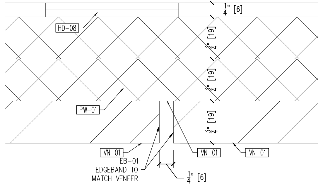
08 DETAIL @ REVEAL 3.02 SCALE: 12" = 12" ARCH. REF.00/0.00
