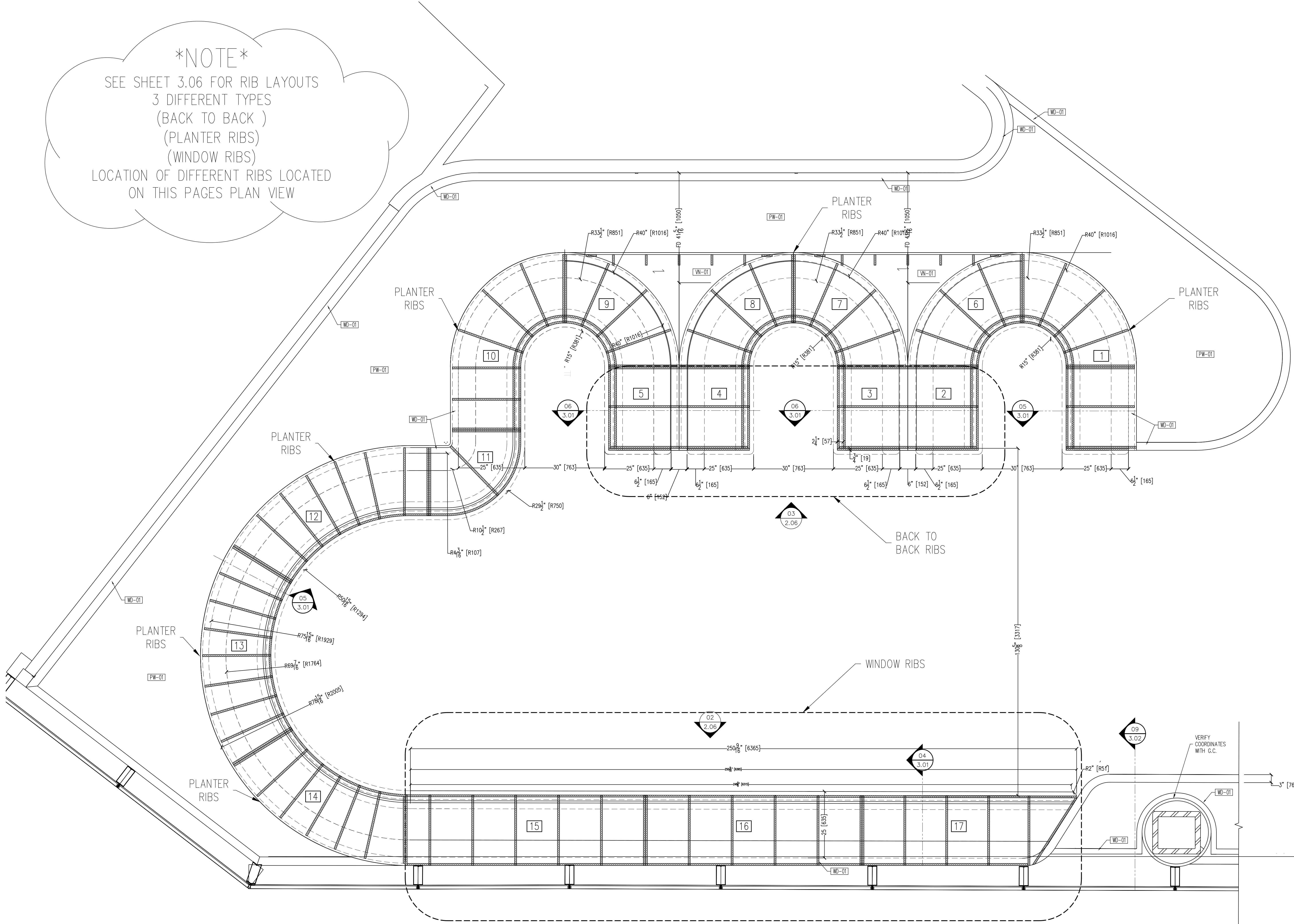
01 PLAN @ UPOLSTERED BANQUETTE SEATING SCALE: 3/4" = 12" ARCH. REF:20/404
