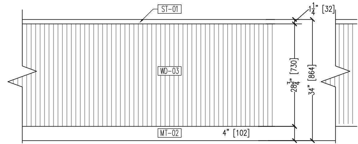
04 ELEVATION @ MARKET COUNTER 2.06 SCALE: 3/4" = 12" ARCH. REF.:0/0.00
