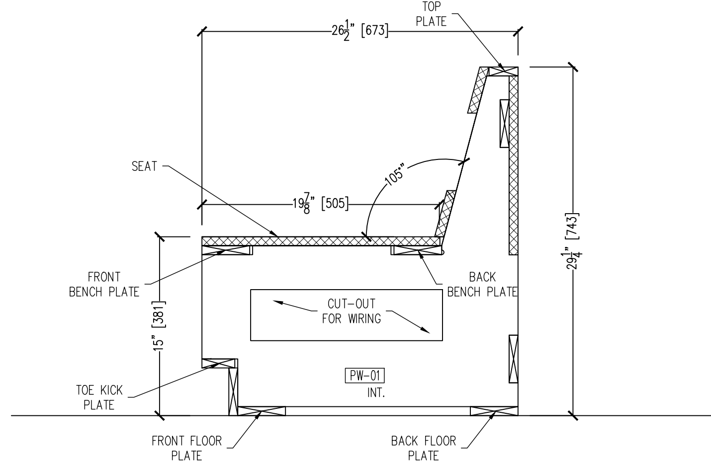
06 SECTION @ WINDOW RIBS WITH PARTS LEGEND 3.06 SCALE: 1 1/2" = 12" ARCH. REF.:32/541
