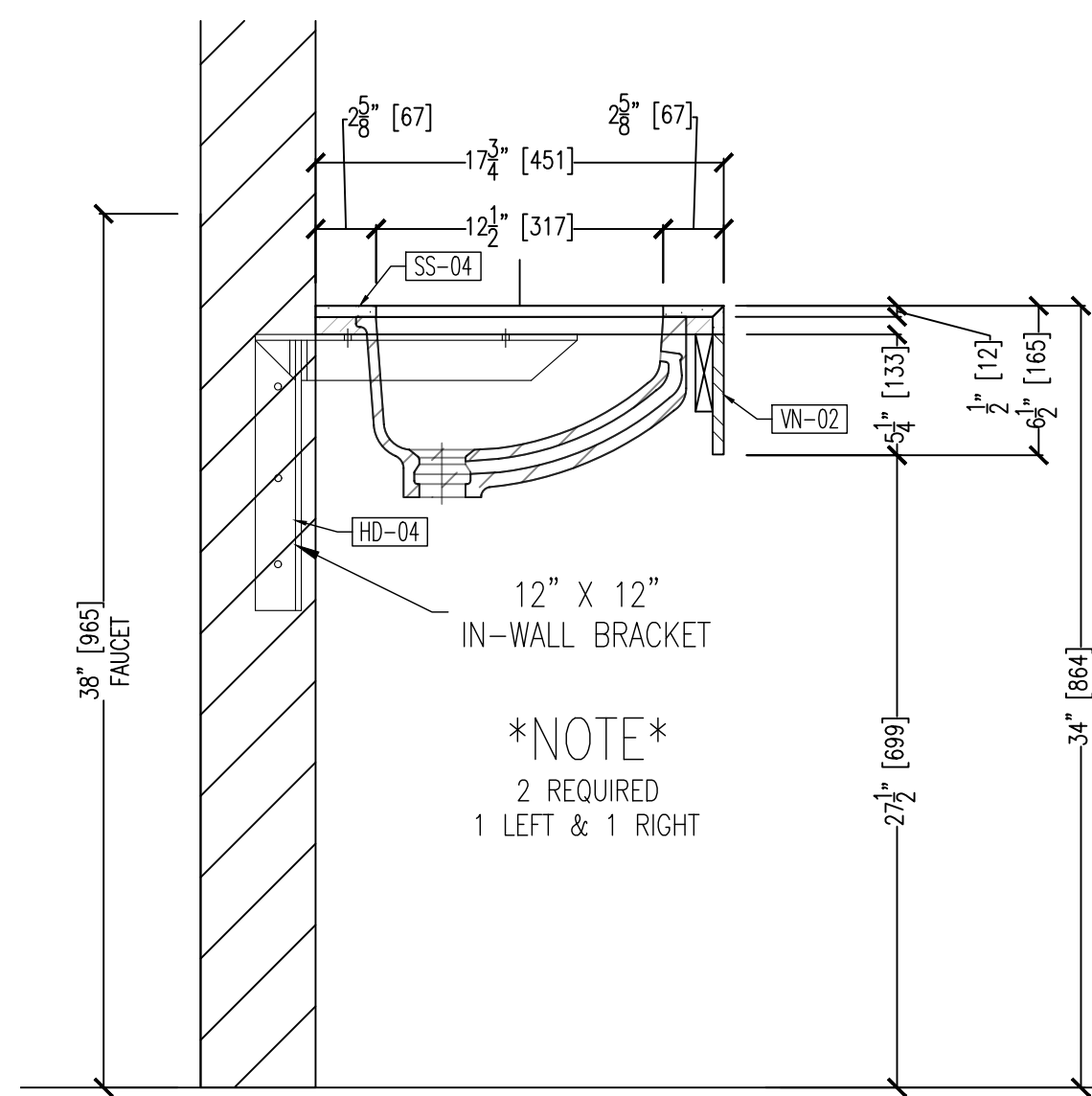
05 SECTION @ ADA BATHROOM 3.03 SCALE: 1 1/2" = 12" ARCH. REF.:31/552
