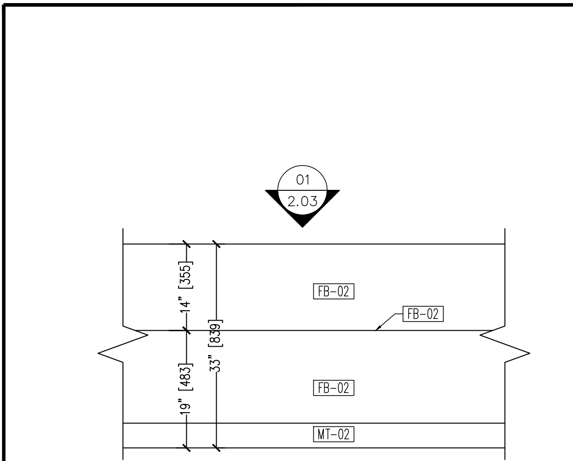
02 ELEVATION @ BANQUETTE 2.06 SCALE: 3/4" = 12" ARCH. REF.:30/200
