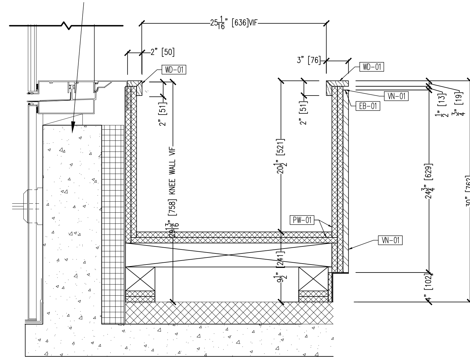
09 SECTION @ PLANTER 3.02 SCALE: 1 1/2" = 12" ARCH. REF.22/541
