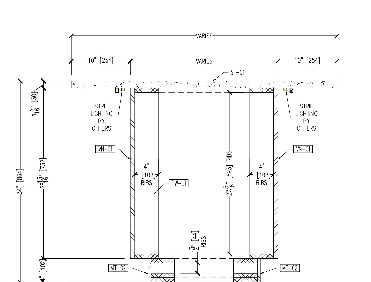
04 SECTION @ MARKET ISLAND 3.03 SCALE: 1 1/2" = 12" ARCH. REF.:20/552
