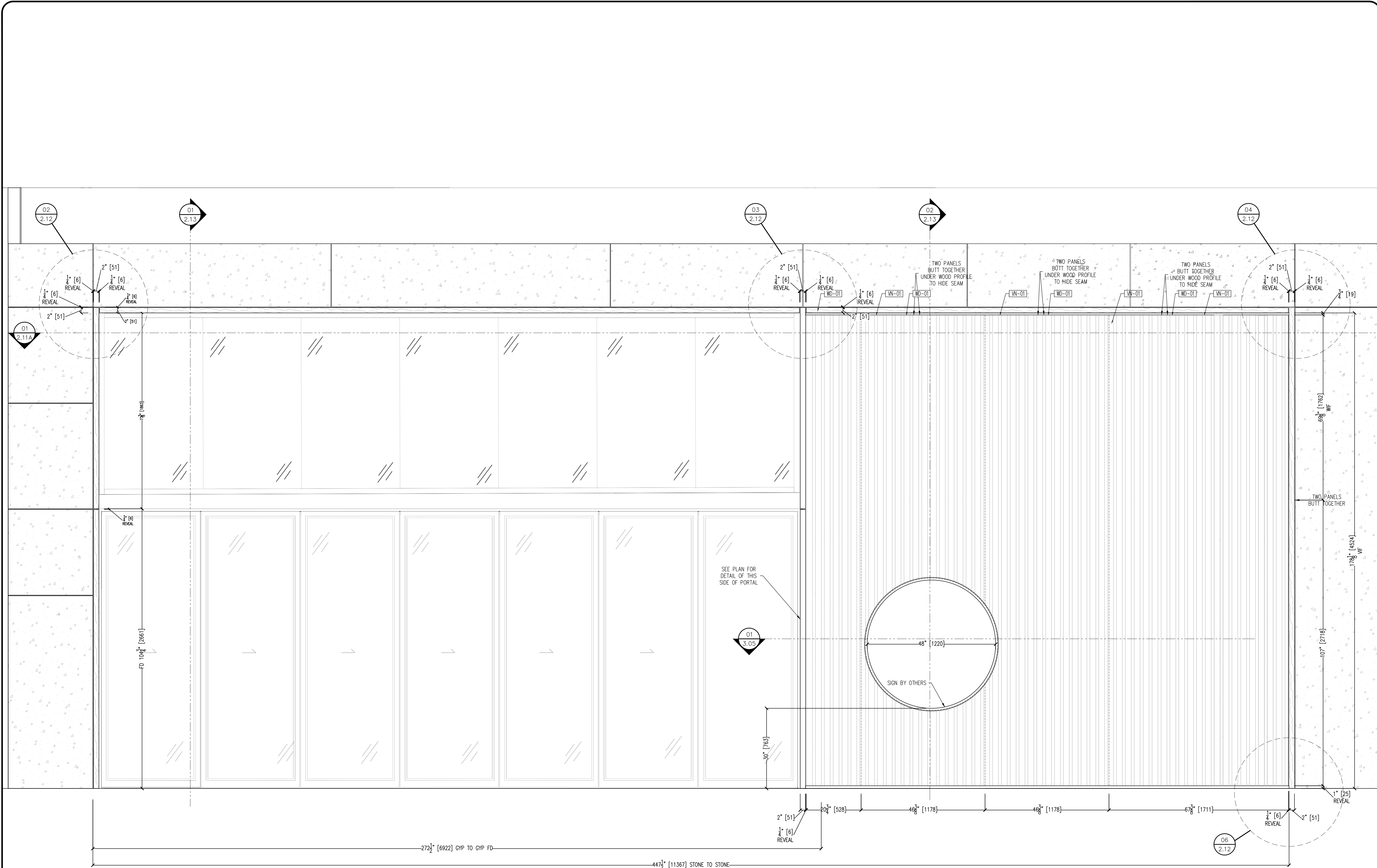
01 ELEVATION @ MARKET ENTRY — LIVING ROOM SIDE 2.11 SCALE: 3/4" = 12" ARCH. REF: 20/201
