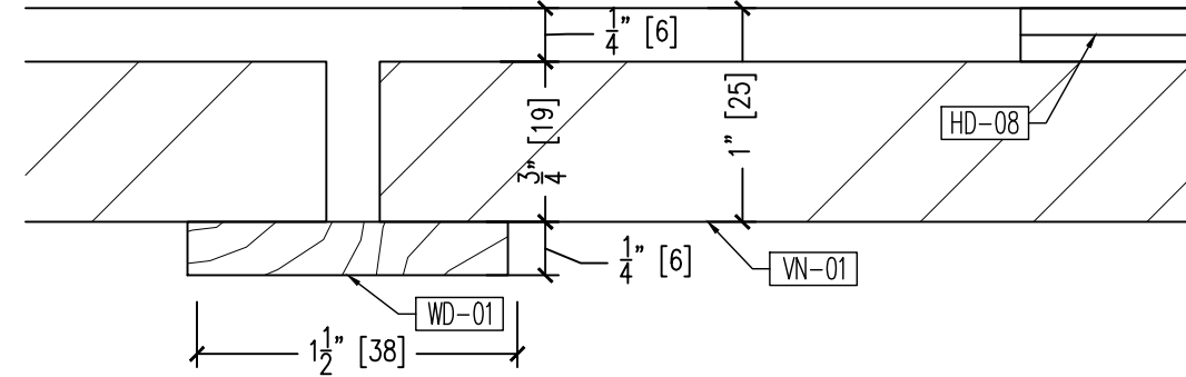
06 DETAIL @ REVEAL 3.02 SCALE: 12" = 12" ARCH. REF.00/0.00
