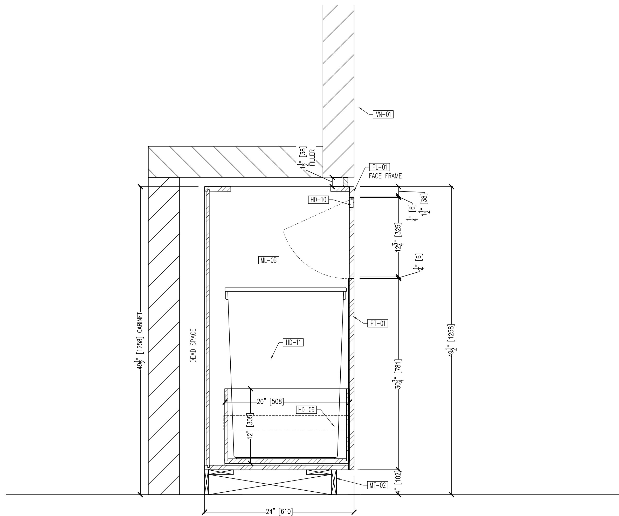
04 SECTION @ MARKET TRASH 2.17 SCALE: 1 1/2" = 12" ARCH. REF.:12/502
