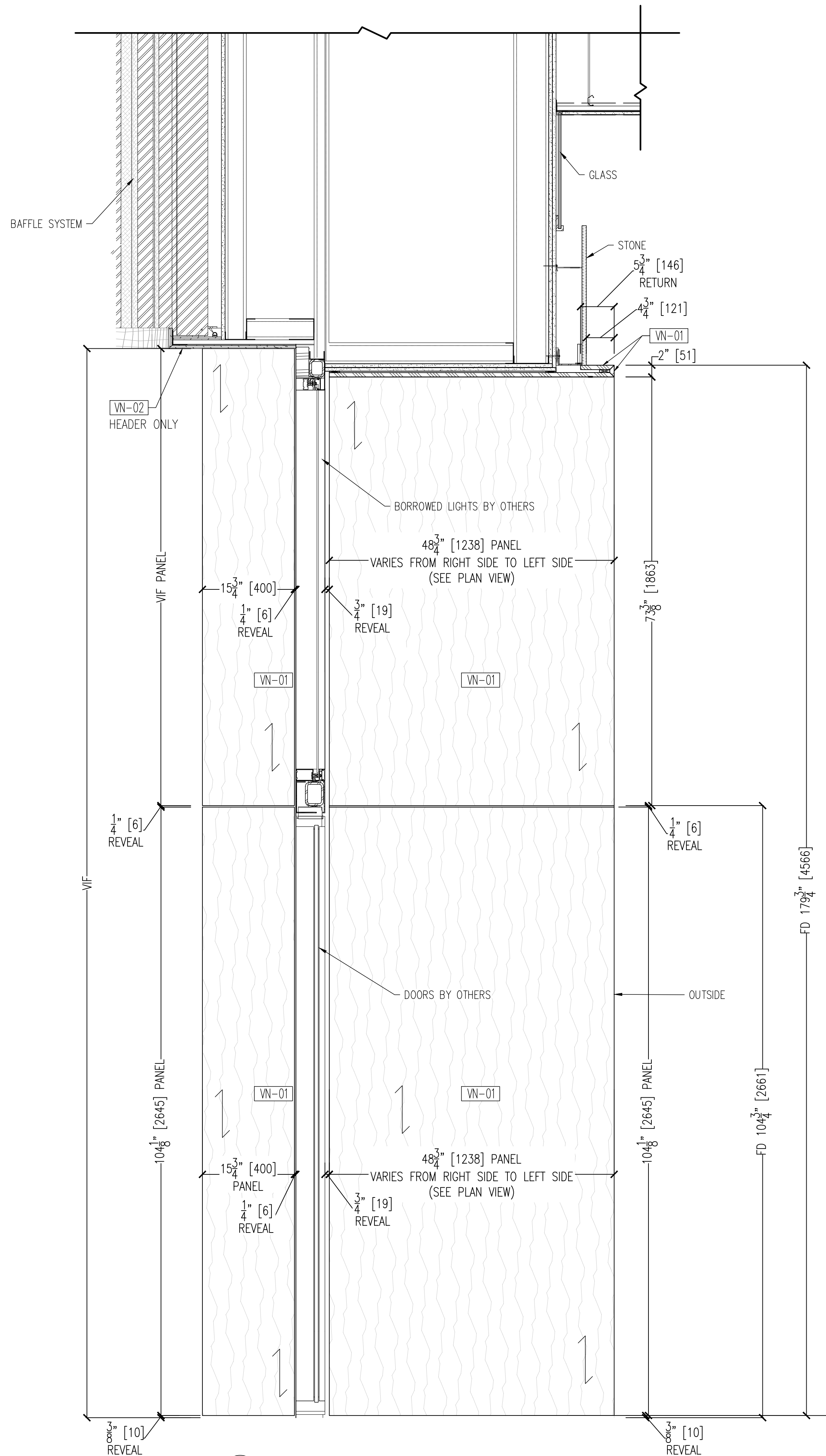
01 SECTION @ ENTRY WALL SIDE PANELS & SOFFIT 2.13 SCALE: 1" = 12" ARCH. REF.:
