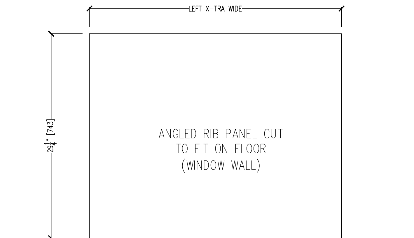
09 SECTION @ ANGELED RIB - CUT TO FIT ON FLOOR 3.06 SCALE: 1 1/2" = 12" ARCH. REF.:32/541
