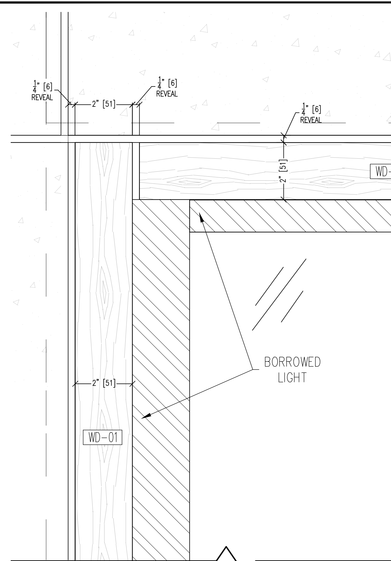
02 BLOW-UP SECTION @ BORROWED LIGHT 2.12 SCALE: 6" = 12" ARCH. REF.:
