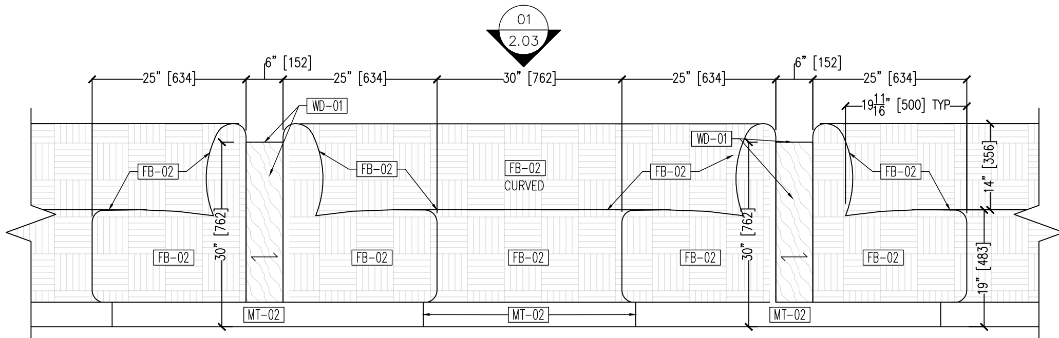
03 ELEVATION @ BANQUETTE 2.06 SCALE: 3/4" = 12" ARCH. REF.:10/542
