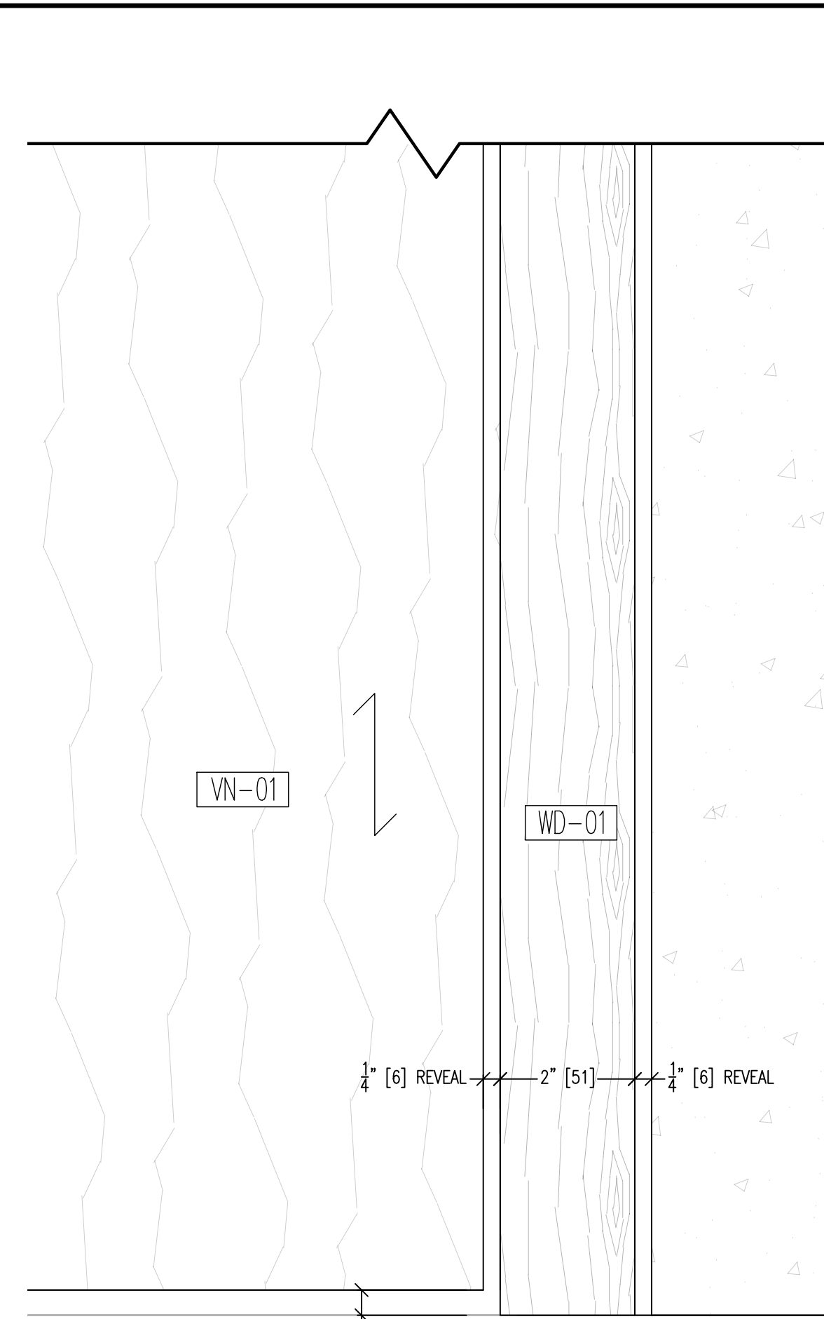
06 BLOW-UP SECTION @ RIGHT END (BOTTOM) 2.12 SCALE: 6" = 12" ARCH. REF.:
