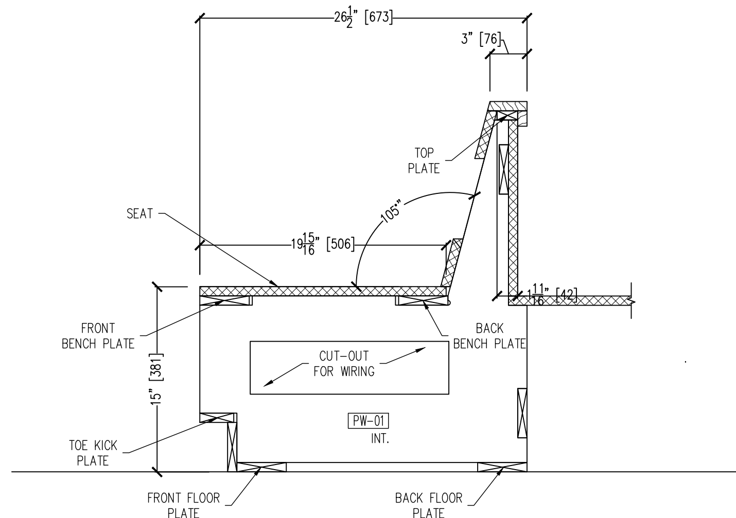
04 SECTION @ PLANTER RIBS WITH PARTS LEGEND 3.06 SCALE: 1 1/2" = 12" ARCH. REF.:32/541
