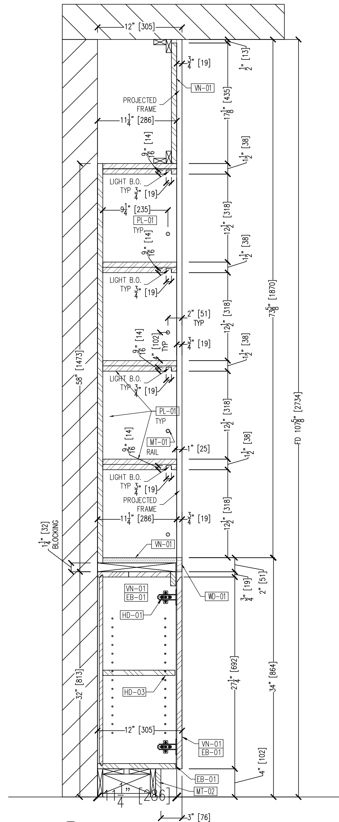
05 SECTION @ GRAB & GO SHELVING 3.02 SCALE: 1 1/2" = 12" ARCH. REF.10/552
