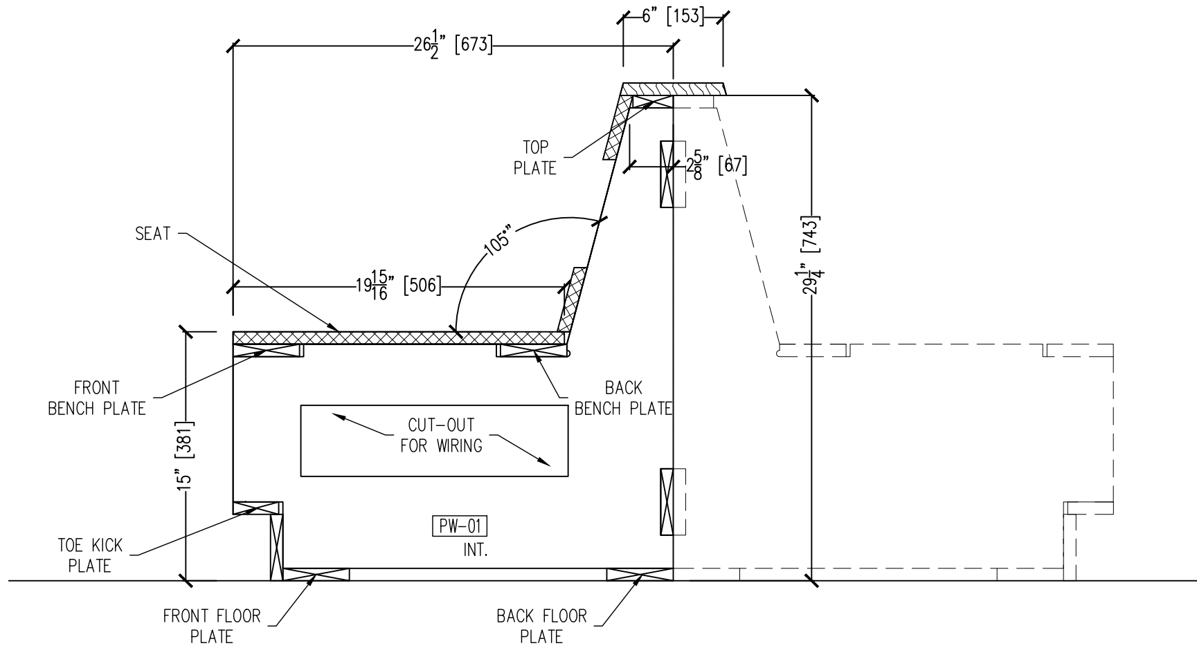
02 SECTION @ BACK TO BACK RIBS WITH PARTS LEGEND 3.06 SCALE: 1 1/2" = 12" ARCH. REF.:32/541
